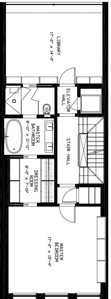
SECOND FLOOR
