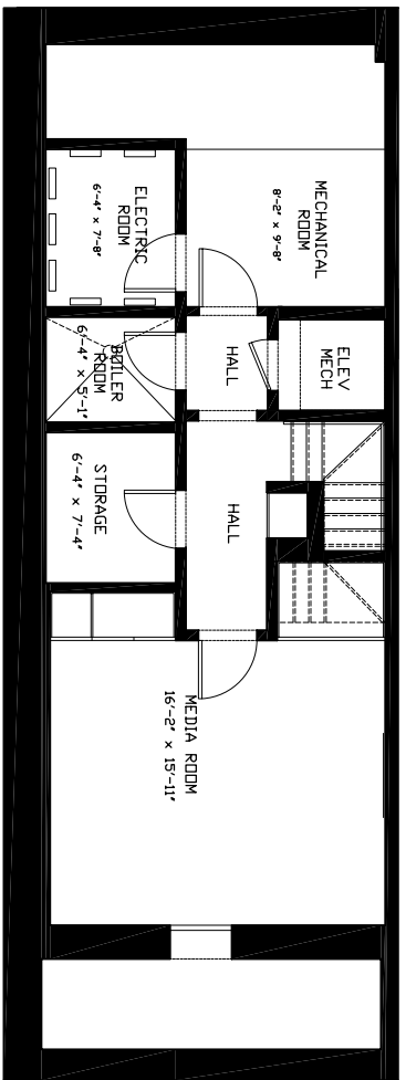
CELLAR
